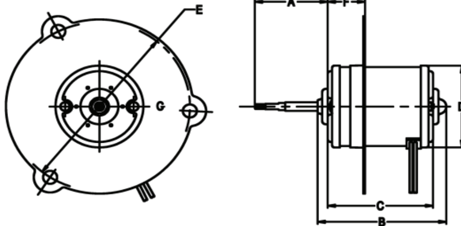
Dimension Chart Blower Motor/Rad Fan Motors
