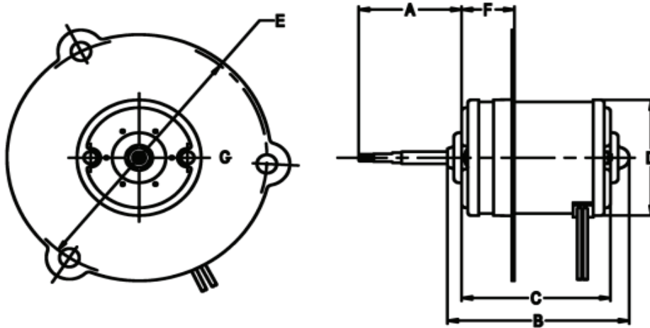
Dimension Chart Blower Motor/Rad Fan Motors
