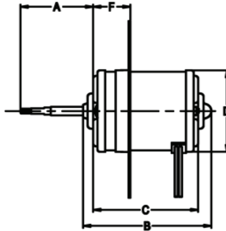
Dimension Chart Blower Motor/Rad Fan Motors
